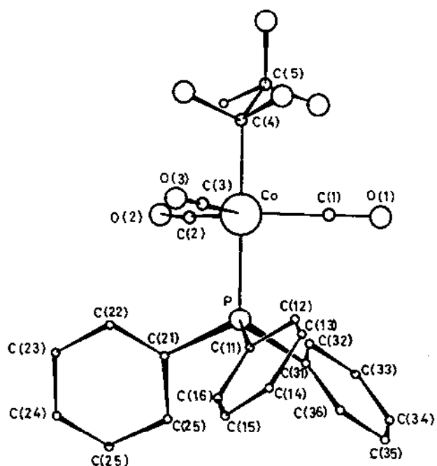
Fig. 3. The X-ray structure of \text{HCF}_2\text{CF}_2\text{Co}(\text{CO})_3\text{PPh}_3 [77].
