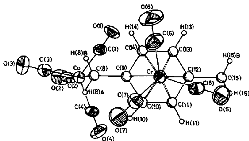
Fig. 2. The X-ray structure of \eta^1\text{-}[\eta^6\text{-(4-MeC}_6\text{H}_4\text{CH}_2\text{)}\text{Cr(CO)}_3\text{]Co(CO)}_4 [8].
