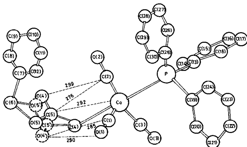
Fig. 4. The X-ray structure of \text{PhCH}_2\text{OOCCH}_2\text{Co}(\text{CO})_3\text{PPh}_3 [2].
